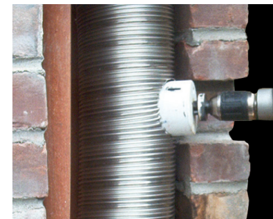
7. If needed, cut Universal Take-off hole into Ventinox.
