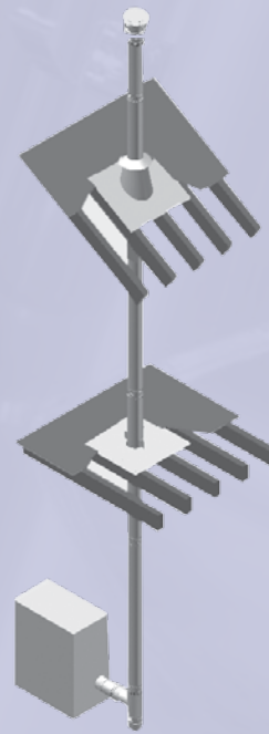
DuraSeal Double Wall (DSD) Vertical Through-the-Roof Installation
